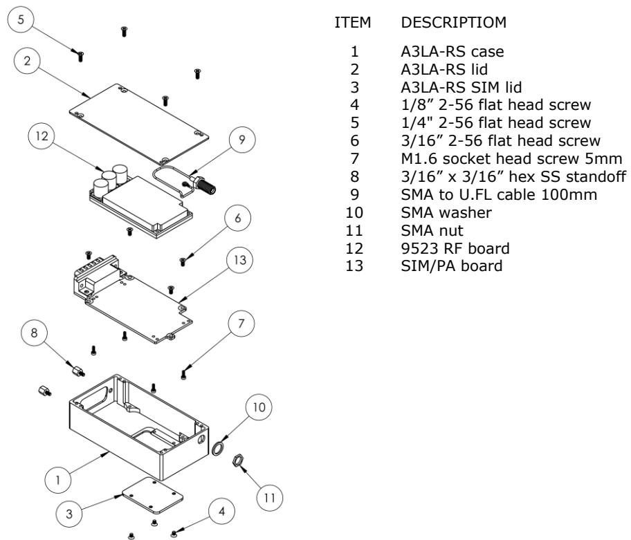
Figure 7. Exploded view of the A3LA-RS.
