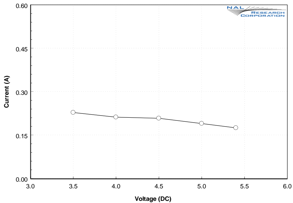
Figure 4. Average current drawn during an SBD transmission.
