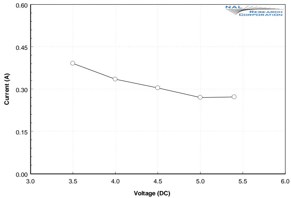
Figure 3. Average current drawn during a data switch call.
