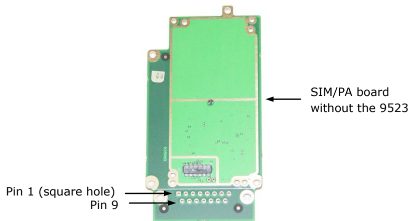
Figure 9. Picture of the SIM/PA board without the 9523.
