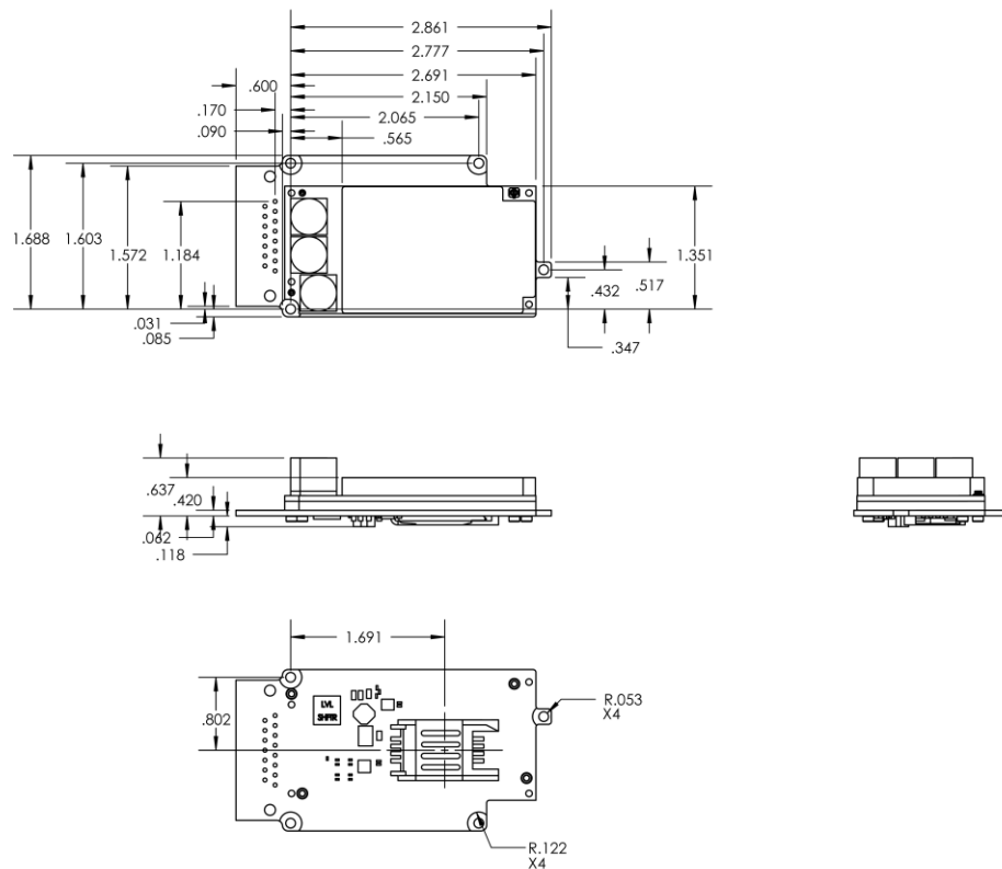
Figure 8. A3LA-RSP comprised mainly of items 12 and 13 (dimensions are in inches).
