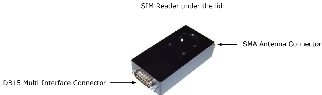
Figure 1. Iridium Satellite Modem A3LA-RS.
