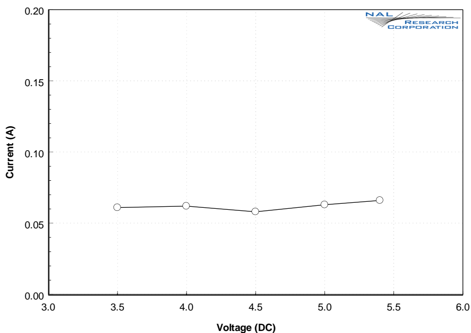
Figure 2. Average current drawn during standby.
