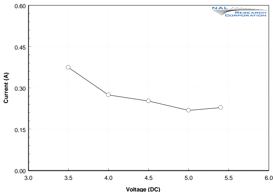
Figure 5. Average current drawn during an SMS transmission.
